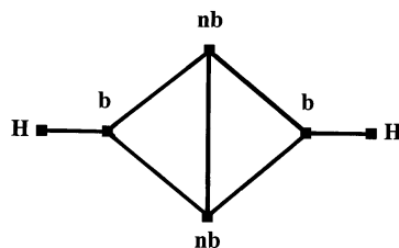
Fig. 4. The planar graph representation of the VSCC graph of water (Fig. 3). This graph has six vertices (squares), seven edges and three faces. A vertex corresponds to a maximum in L(\mathbf{r}) , an edge to a (3, -1) CP and a face to a (3, +1) CP. The two non-bonding vertices (nb, top and bottom) are linked to each other and to both bonding vertices of oxygen (b, left and right).
