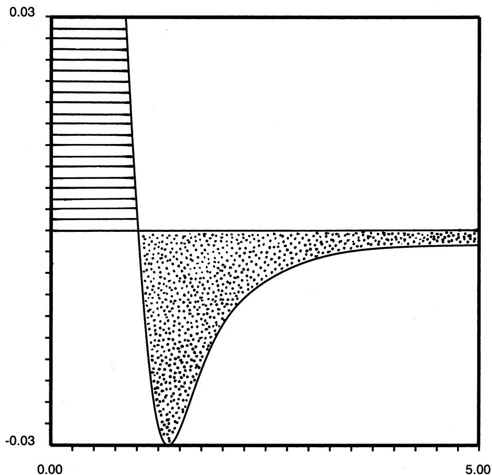
Fig. 2. A truncated representation of L(r) (au) versus the radial distance (au) from the nucleus for a free hydrogen atom, showing two distinct regions. The hatched region is a spherical shell of (electronic) charge concentration (VSCC), and the dotted region is a spherical shells of charge depletion (VSCD).
